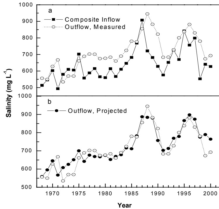
Fig. 7. Estimated salinity of the inflow, the estimated and the recorded salinity of the outflow from Amistad International Reservoir.
