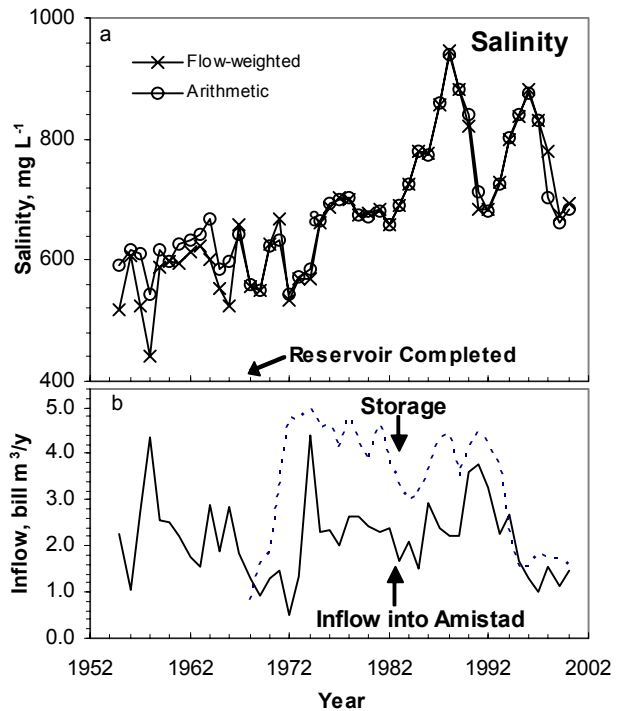
Fig. 2. Changes in salinity, inflow into and storage at Amistad Reservoir.
