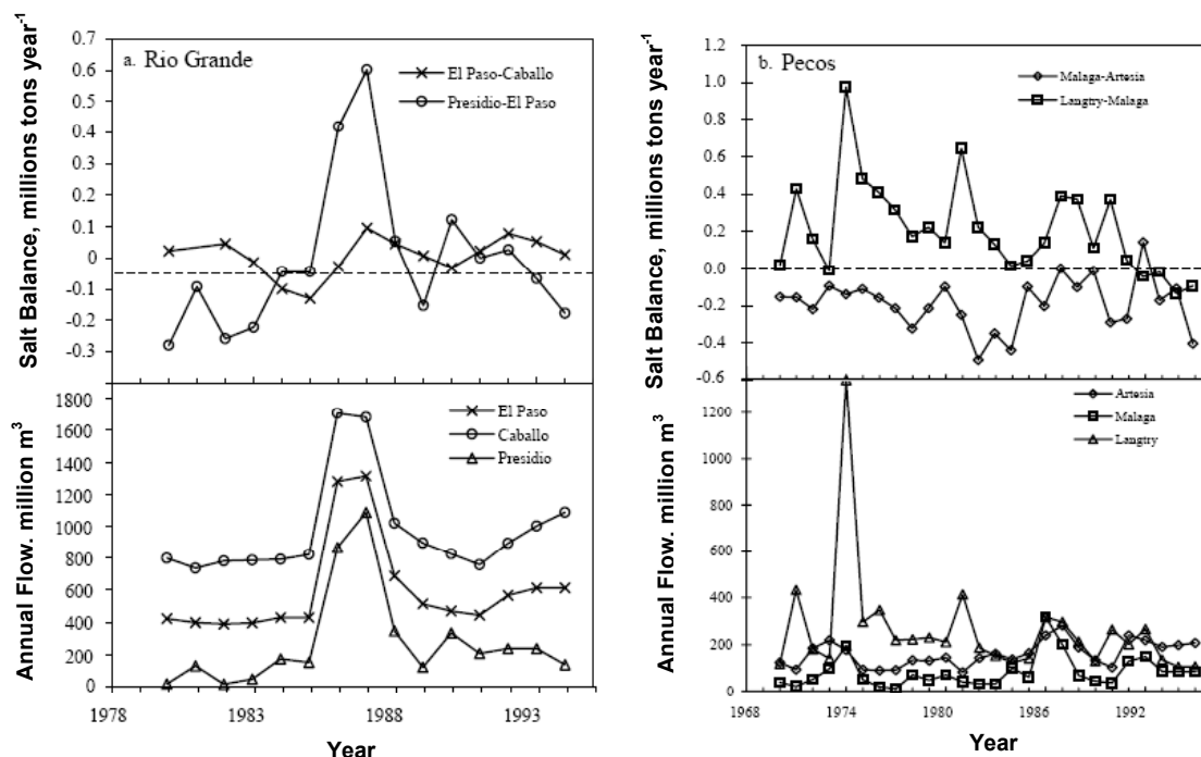
Fig. 5. The annual salt balance and the streamflow measured at three locations.
