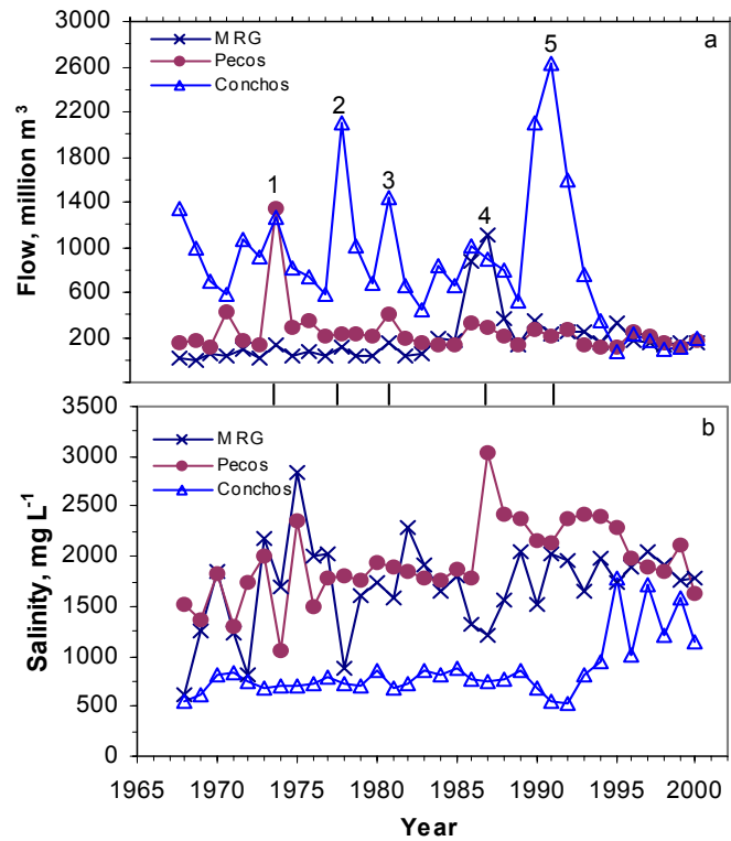
Fig. 3. Flow and salinity of the main tributaries entering Amistad Reservoir.
