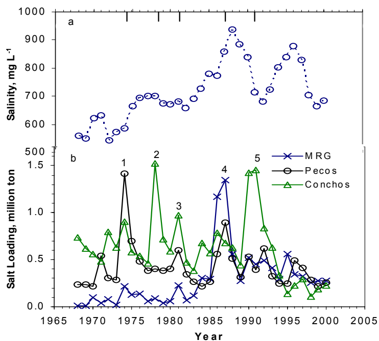
Fig. 4. Salt loading from the main tributaries, and salinity of the reservoir.
