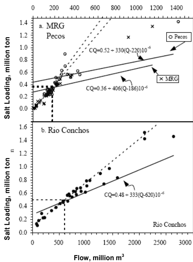
Fig. 6. The relationship between salt loading and flow at these tributaries.
