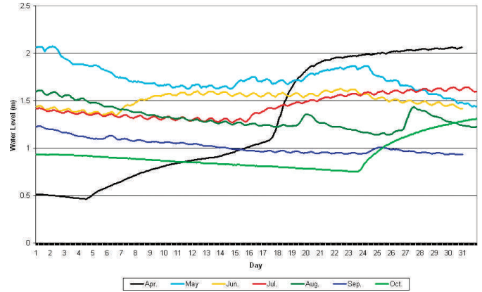
Figure 1. Growing season hourly water levels for well A1 in 2001 (pretreatment).
